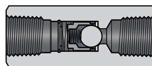
Dual Seal
