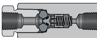
Soft Seat
